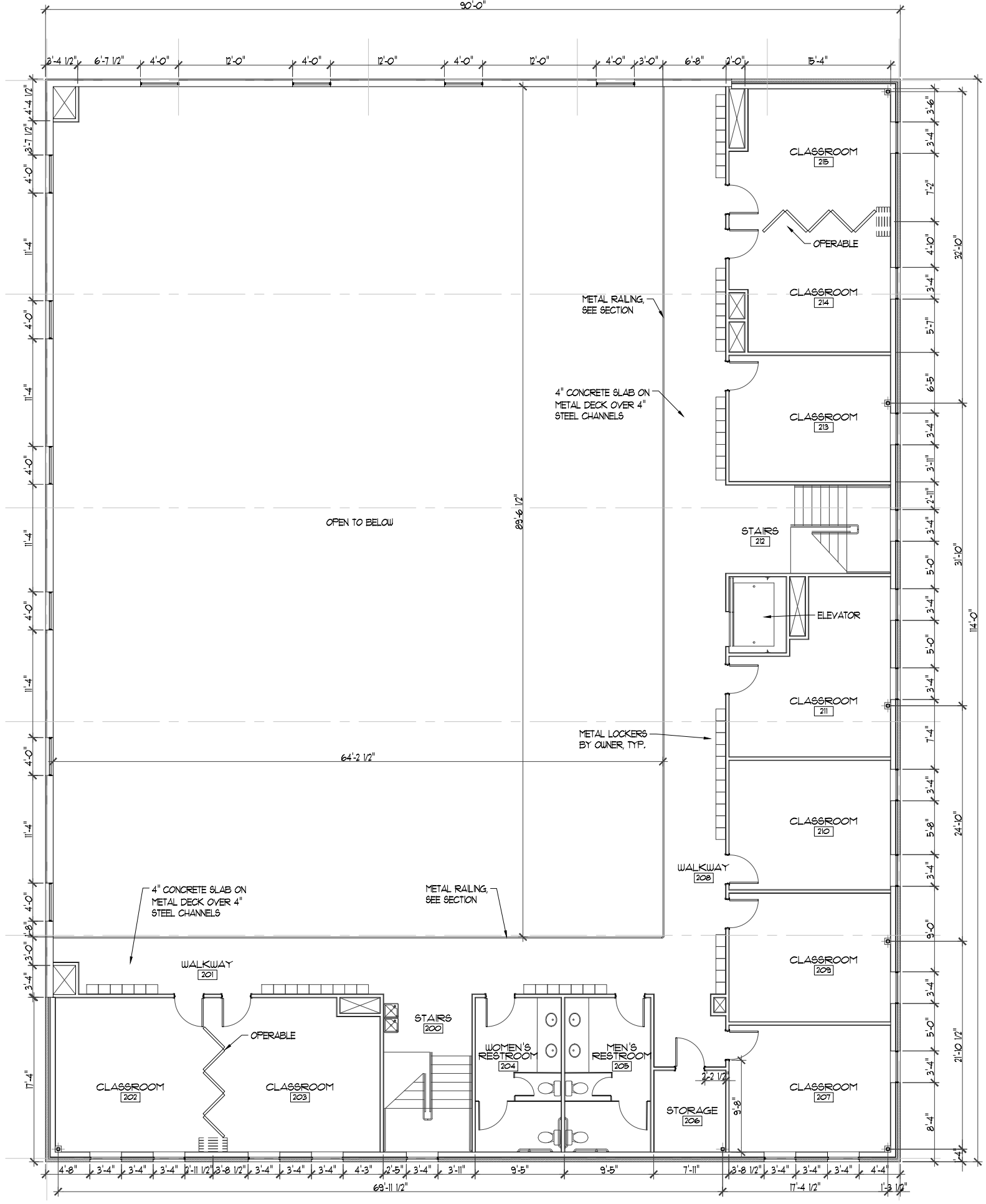
2 A3.1 UPPER LEVEL FLOOR PLAN SCALE: 1/8"=1'-0"
